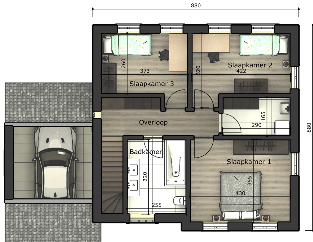
VERDIEPING Opp. verdieping 76 m 2
