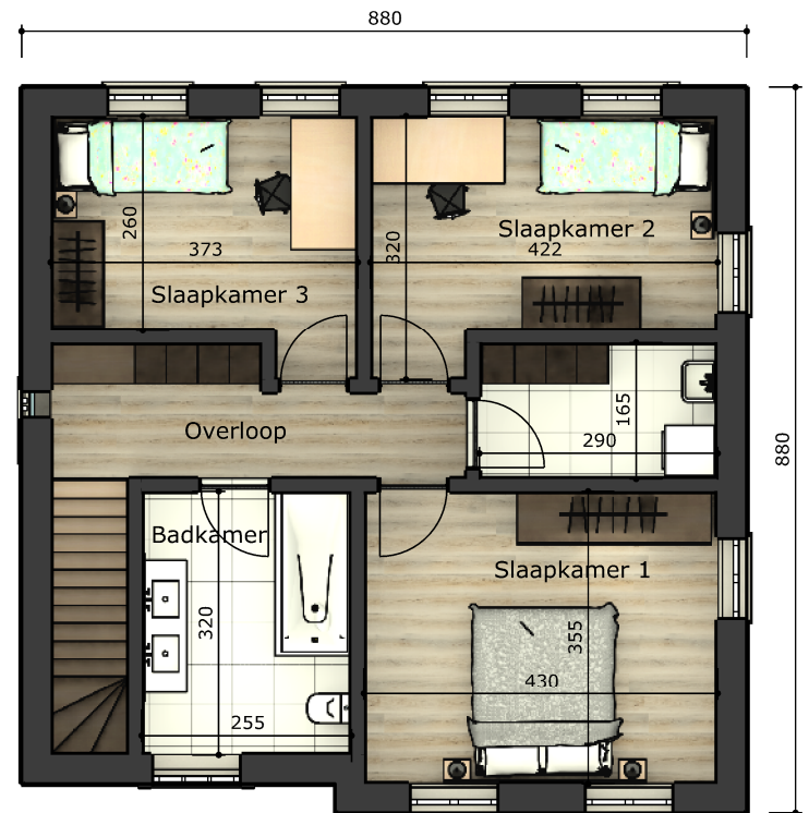
VERDIEPING Opp. verdieping 76 m 2
