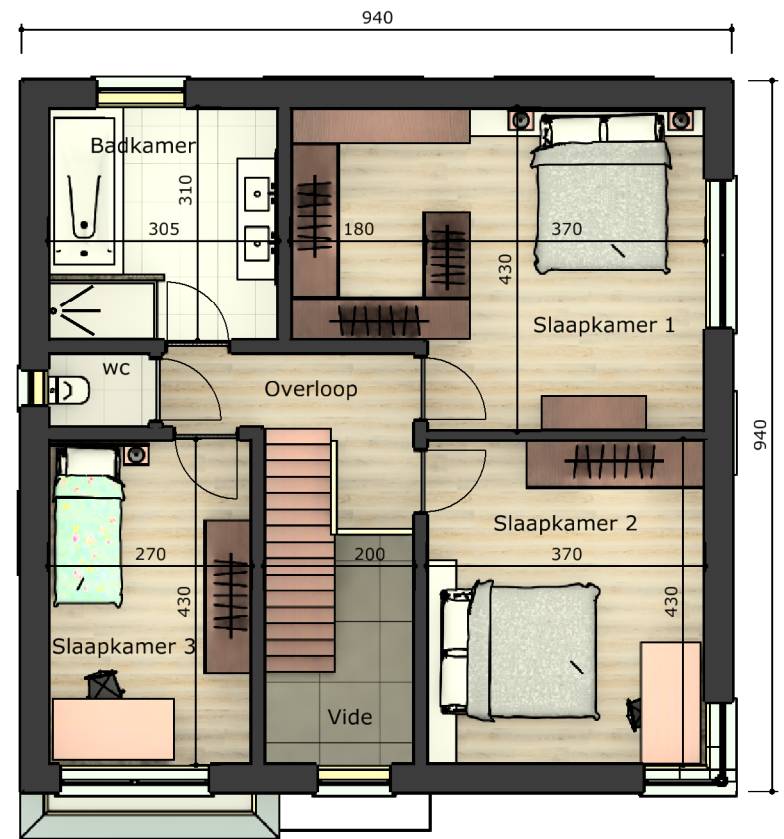
VERDIEPING Opp. verdieping 88.36 m 2
